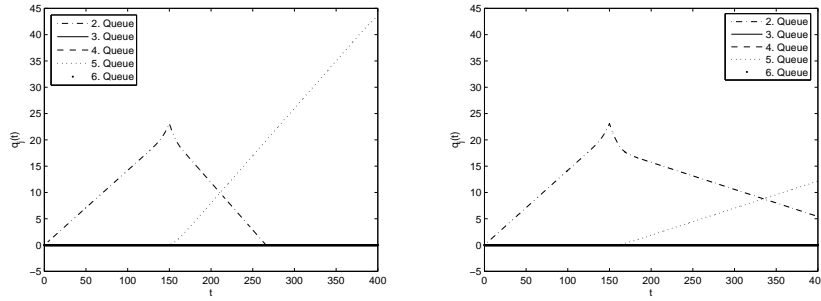
Figure 17: Evolution of queues for the initial situation with \alpha_1 = 1 (left) and in the optimum \alpha_1 = 0.819004 (right)
