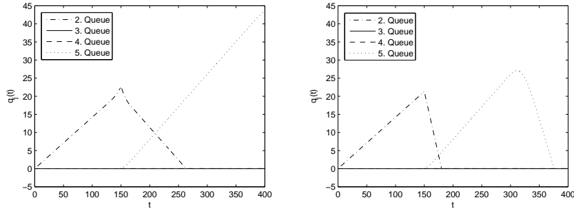
Figure 15: Amount of parts in queues q_j(t) , j = 2, 3, 4, 5 for default (left) and optimal (right) velocity
