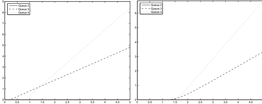
Figure 12: Evolution of queues in the case of unrestricted (left) and length restricted (right) queues.
