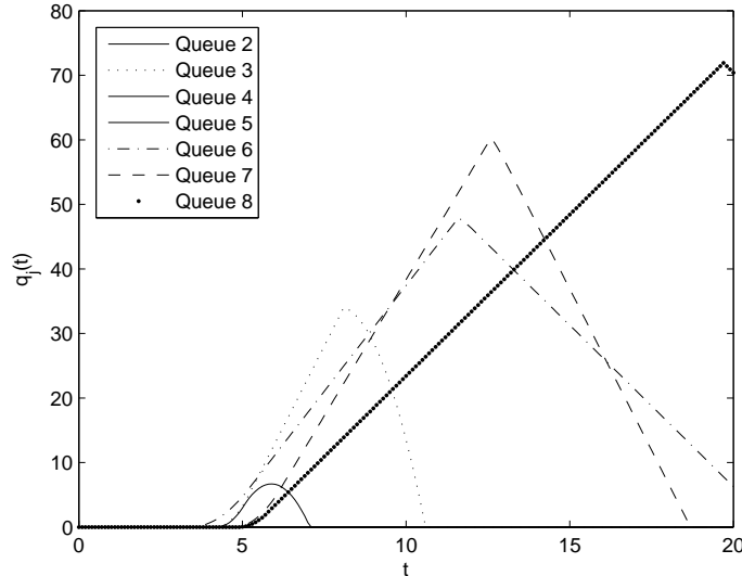
Figure 7: Amount of parts in each queue for optimal distribution rates \alpha_1^{opt} = 1 and \alpha_2^{opt} = 0.385097 . Queue 4 and Queue 5 remain empty.
