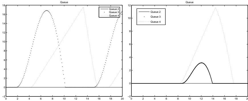
Figure 10: Evolution of the queues in test case one for the default (left) and optimal (right) velocities
