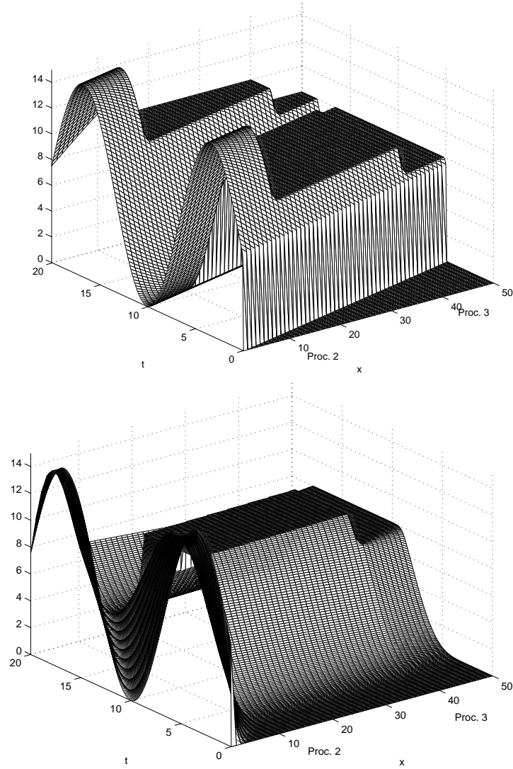
Figure 11: Evolution of the fluxes f_j(x, t) in test case one for the default (top) and optimal (bottom) velocities. Processor one is located in 0 \leq x \leq 10 and processor two at 10 \leq x \leq 40
